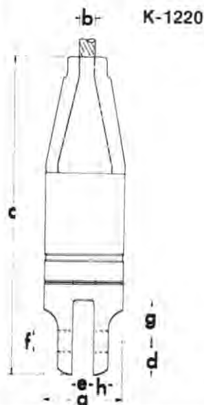
CLEVIS SHANK
