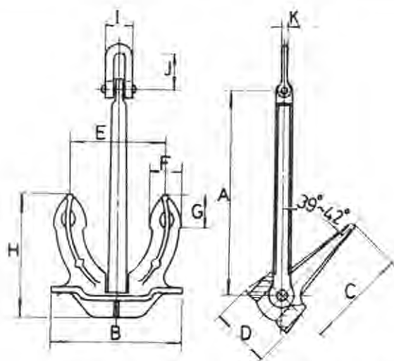
DIMENSIONS (mm)
