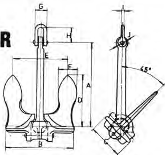
DIMENSIONS (mm)
