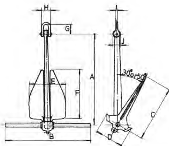
DIMENSIONS (mm)
