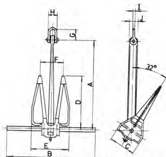
DIMENSIONS (mm)
