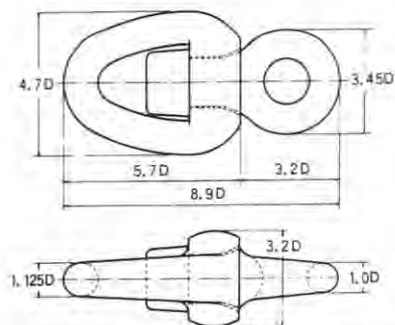
Swivel = SW
