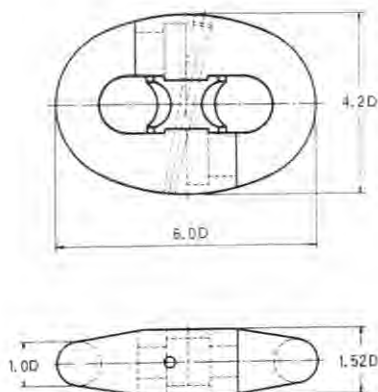
Swivel = SW
