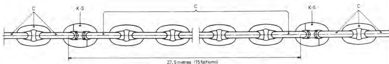
Connection with kenter shackles
