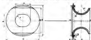
SINGLE BOW - BULWARK MOUNTING IN FLAT PLATE
