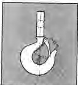
Shank Hook Dimensions with Latch Assembled
